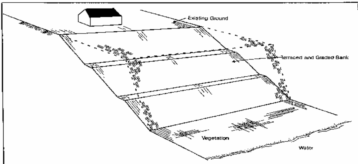
Figure 6. Grading and terracing.
