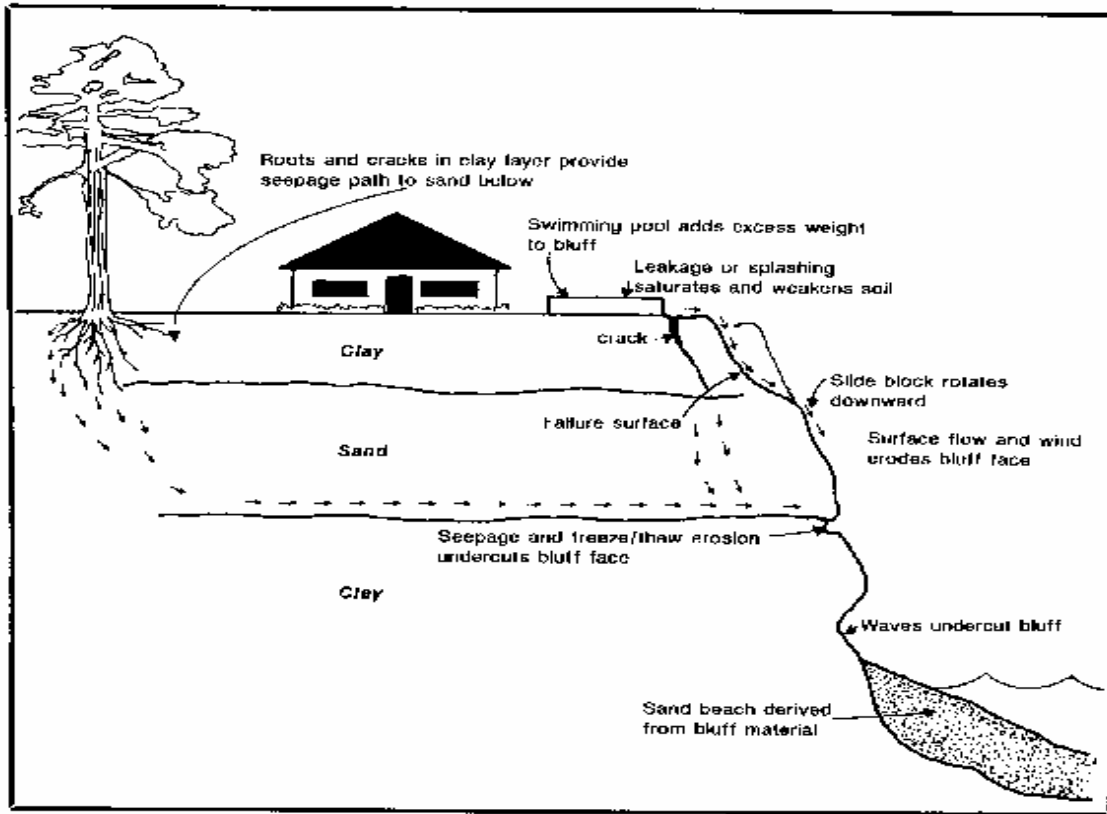
Figure 4. The combination of wave and groundwater erosion on a high bank.
