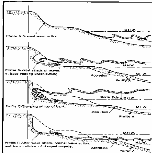
Figure 1. Wave erosion and transportation of sediments along a beach.
