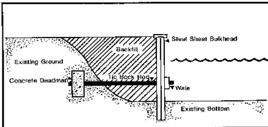
Figure 10. Basic design of a sheet pile bulkhead.
