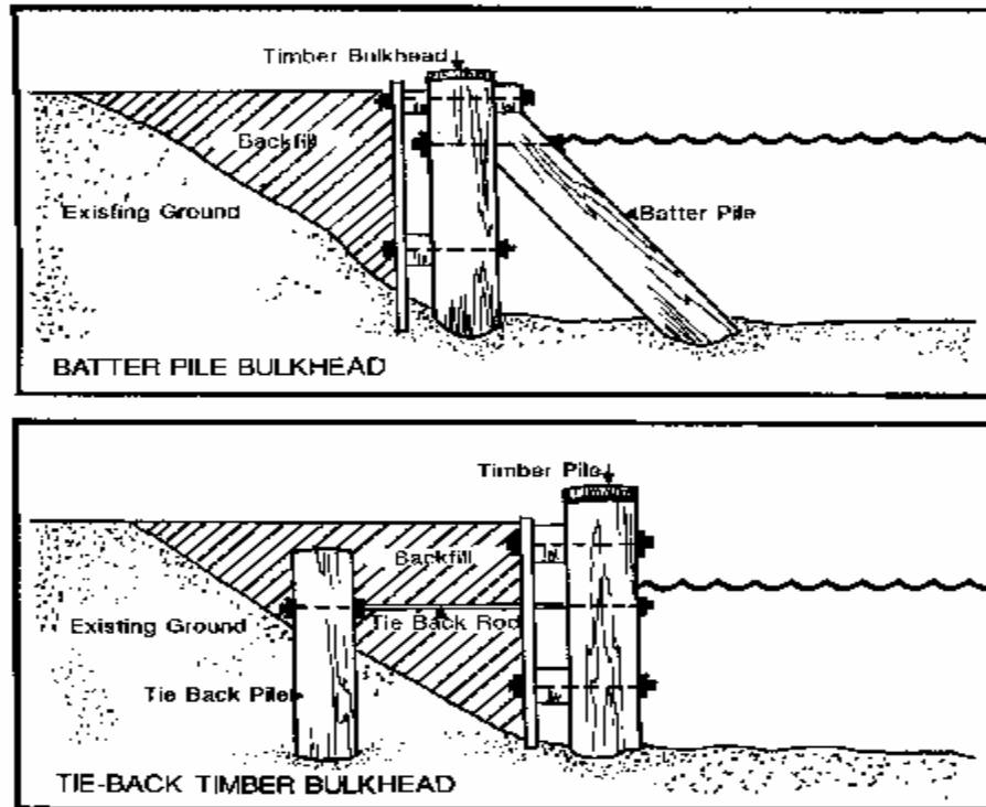
Figure 12. Profile view of the two types of post-supported bulkheads.
