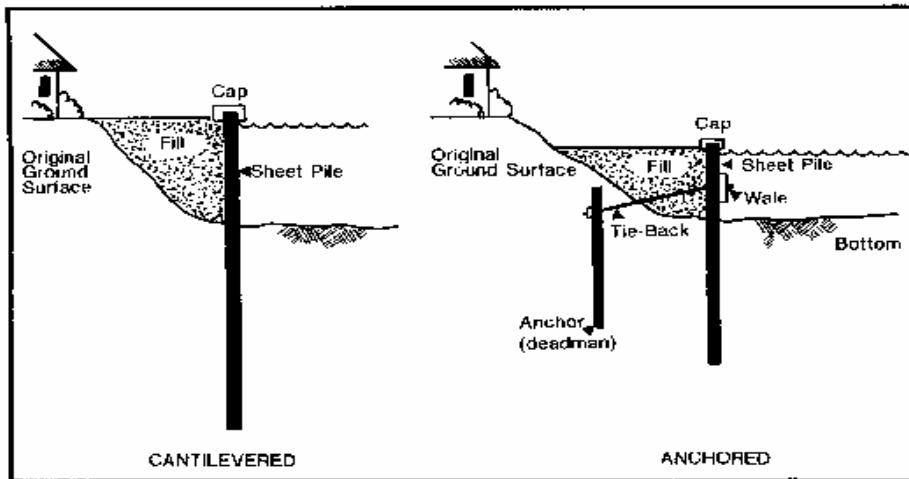
Figure 11. Cantilevered and anchored sheet pile bulkheads.
