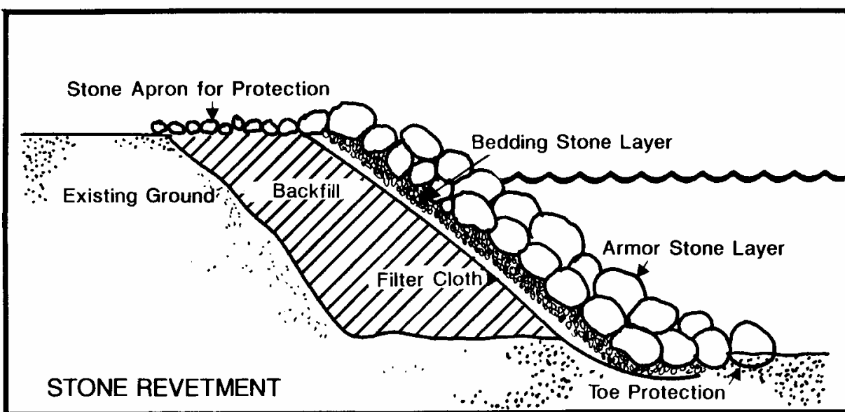
Figure 8. Profile of a stone revetment.
