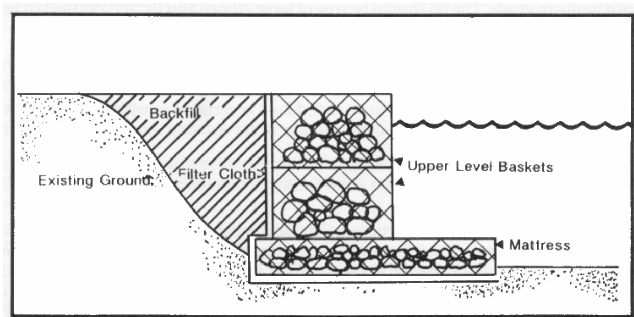
Figure 9. Gabion (used as a wall).
