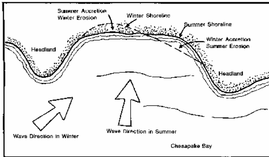
Figure 2. Seasonal changes in erosion and depositional patterns due to changing wave direction exposing new surfaces.
