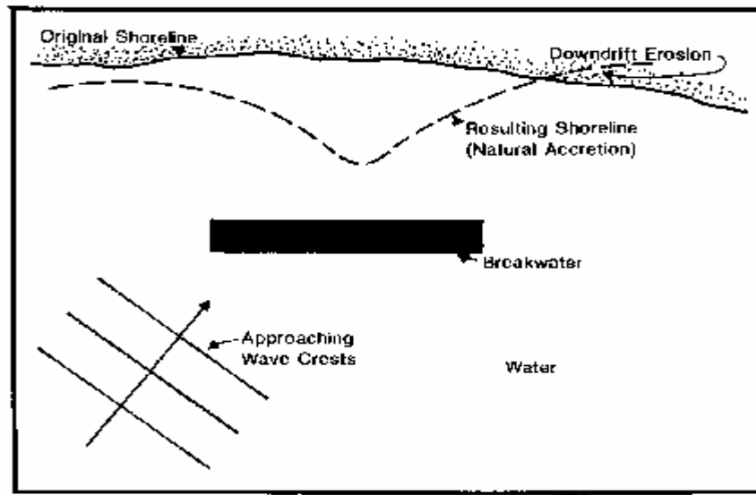
Figure 14: Breakwater exhibiting the deposition of sand on the leeward side.
